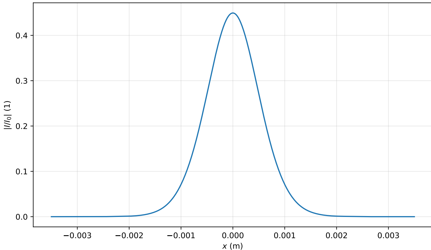
Intensity profile I(x, y = 0, z = 3.184m)/I_0 , P_{in}=0.4P_{cr} , artificial time
